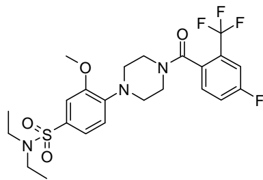
PC-6158901, DMSO-d6
